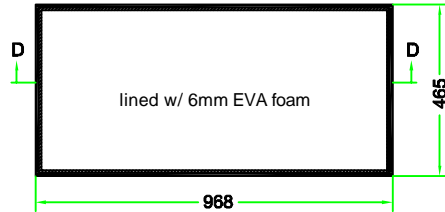
TOP VIEW OF COVER
