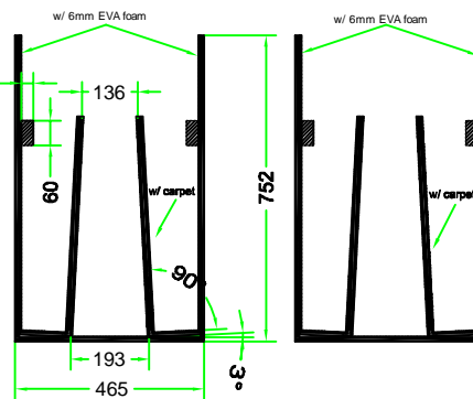
B-B VIEW
